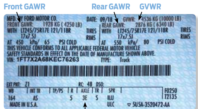
Axle Code
